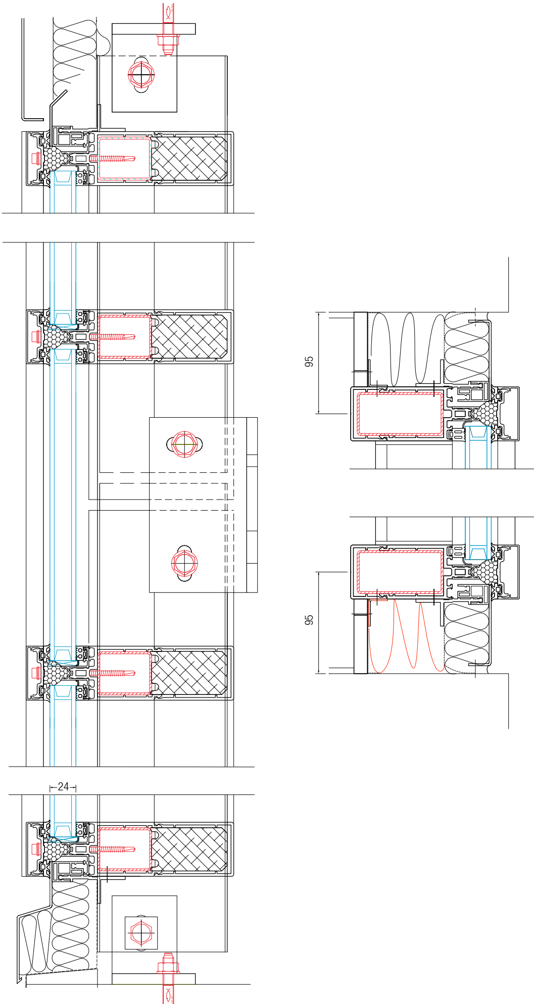
Vertical Section
